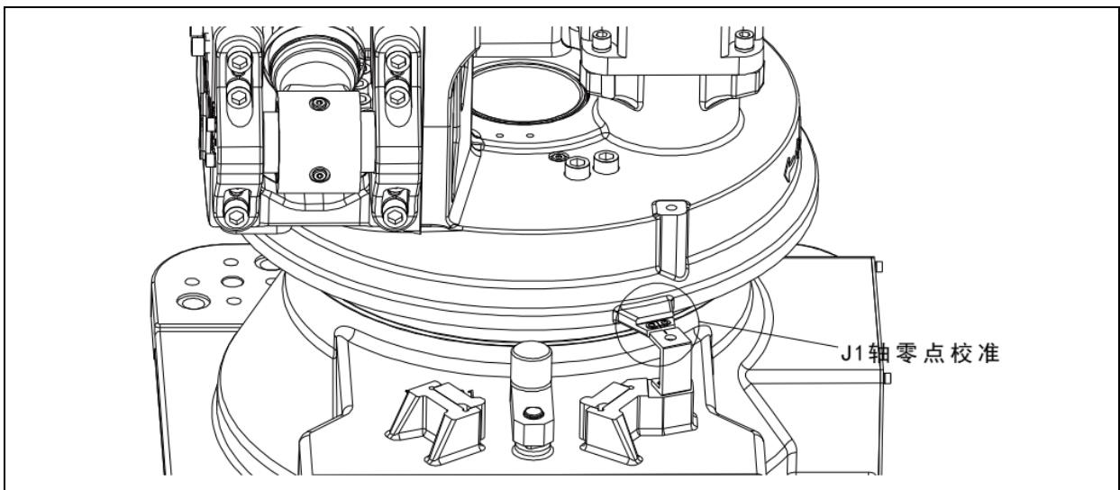
图 6.3 J1 轴零点校准示意图(ER100B-3000, ER130B-3200, ER170B-2650, ER220B-2650)
