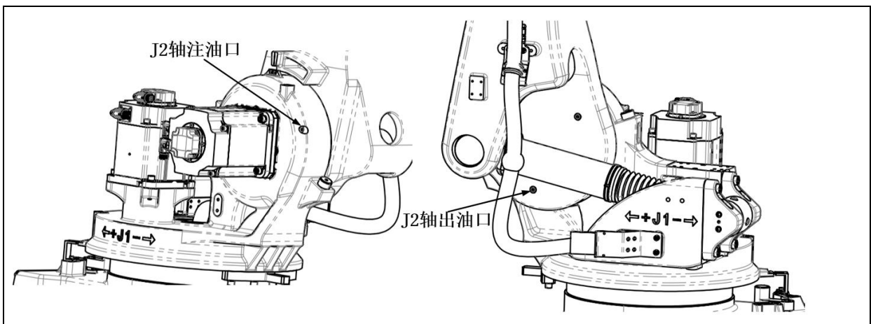
图 5.11 J2 轴注油、出油口 (ER100B-3000, ER130B-3200, ER170B-2650, ER220B-2650)
